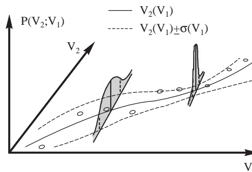
Fig. 1. Illustration of the functions defined in Eq. (3). Each point corresponds to a single conformation \vec{q}_i of the system, being V_1(\vec{q}_i) its x -coordinate and V_2(\vec{q}_i) its y -coordinate. In the z -axis, the probability density of measuring a particular value of V_2 for each value of V_1 . Two normal distributions representing this quantity are shown at arbitrary positions in the x -axis. The continuum line represents the mean V_2(V_1) of the values V_2(\vec{q}) with \vec{q} \in \mathcal{C}(V_1) as a function of V_1 . The broken lines enclose the region where there is the largest probability to find a conformation if a single numerical experiment is performed (around 68% if the distribution of V_2 is assumed to be normal for each V_1 ).
