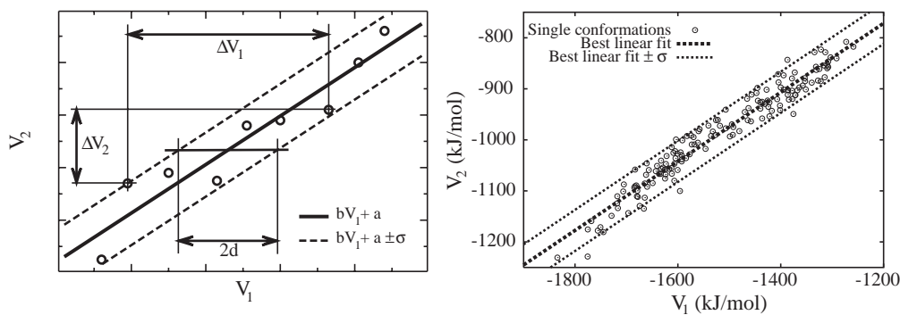
Fig. 2. The graphic on the left is an illustration of the distance criterion. The best linear fit is depicted by a continuum line. The broken lines correspond to the estimated standard deviation of the points in the V_2 direction. The V_1 - and V_2 -energy differences, \Delta V_1 and \Delta V_2 , between two particular conformations, as well as the distance d for \alpha=1 (see Eq. (8)) are also shown. The graphic on the right is a particular example taken from the system studied in Section 3. The difference between the V_1 and V_2 instances is a small modification of the surface of separation between dielectrics. 150 conformations of the investigated protein are shown.
