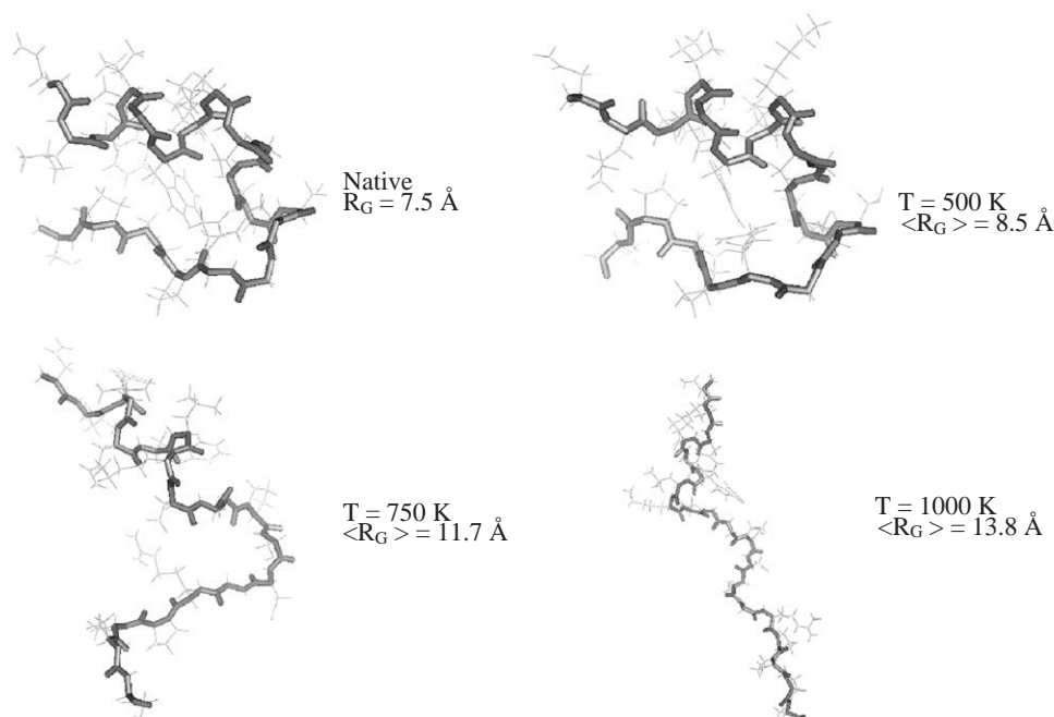
Fig. 4. Example conformations of the studied Trp-Cage protein. The native structure, taken from the Protein Data Bank is shown on the upper left corner. From left to right and from top to bottom, three particular conformations arbitrarily chosen from three different sets are depicted in order of decreasing similarity to the folded protein. The average radii of gyration in each set \langle R_G \rangle and the one of the native structure are also presented.
