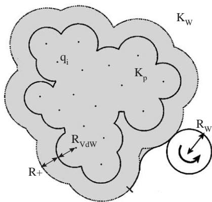
Fig. 3. Dielectric model of the protein. Atomic charges q_i are punctual and located at nuclei. Space is divided in two disjoint regions: the macro-molecule (in gray), with low dielectric constant \kappa_p and the water (in white), with high dielectric constant \kappa_w . The surface of separation between the two media is constructed as described in the text.
