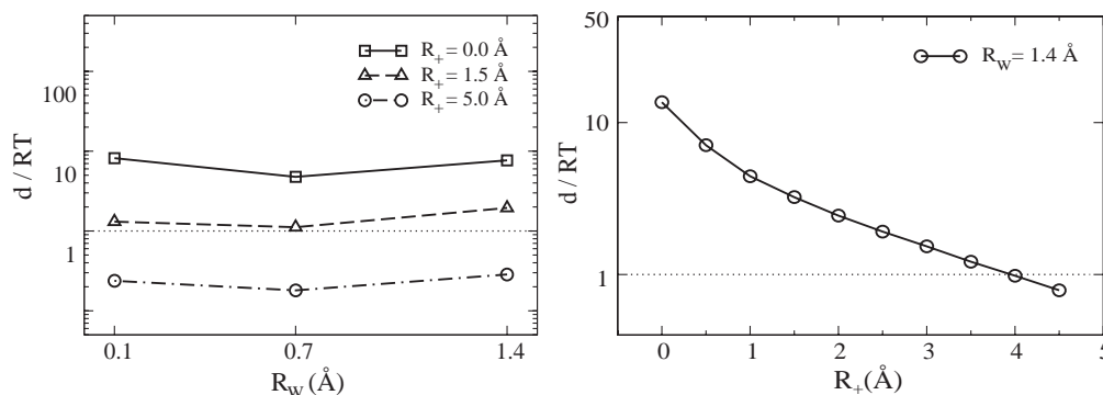
Fig. 6. Distance between instances of the Poisson solvation energy corresponding to different values of the free parameters. The y-axis corresponds to the distance d measured in units of RT (with T=300 K) and the scale is logarithmic. Each point represents the comparison of the energies calculated with the value of the parameters in its x coordinate and the one calculated with the immediately greater value (see text). The graphic on the left shows the results obtained when R_+ is held fixed and R_W is varied. When R_W is kept constant and R_+ is varied, the measured distance d is the one depicted in the graphic on the right.
